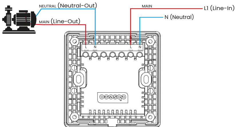
Figure 1: Wiring Diagram
